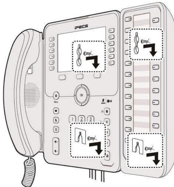
Figure 1.8_Wall Mount Installation
